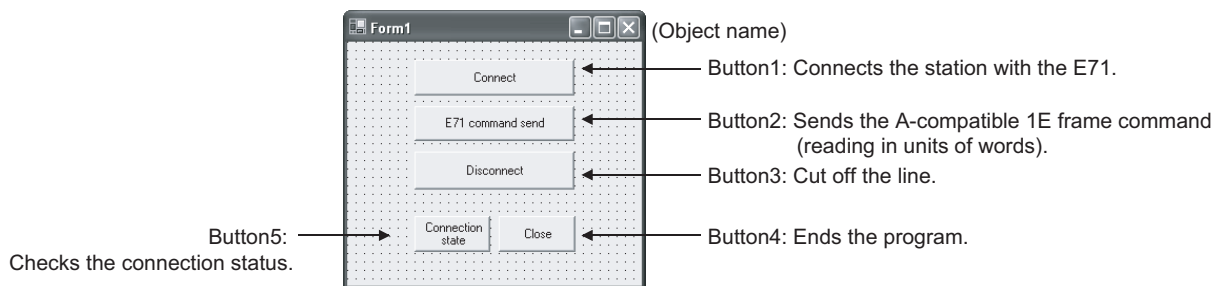
[Window example (Form 1.vb)]
